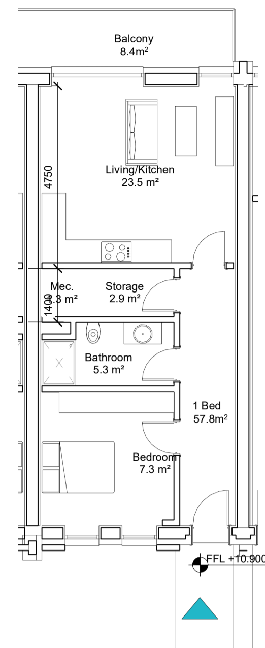
1 TH TYPE 1h (GF) 1 : 100 1B2P 57.8m² - Area 8.4m² - Private Amenity 66.2m² - TOTAL AREA
