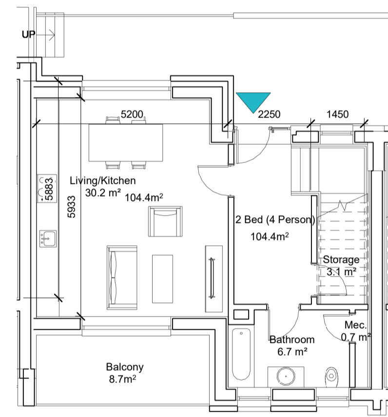
8 TH TYPE 5h (Lv01) 1 : 100 2B4P 104.4m² - Area 8.7m² - Private Amenity 113.1m² - TOTAL AREA
