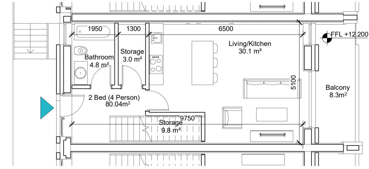
12 TH TYPE 8h (Lv01) 1 : 100 2B4P 80.4m² - Area 8.3m² - Private Amenity 88.7m² - TOTAL AREA
