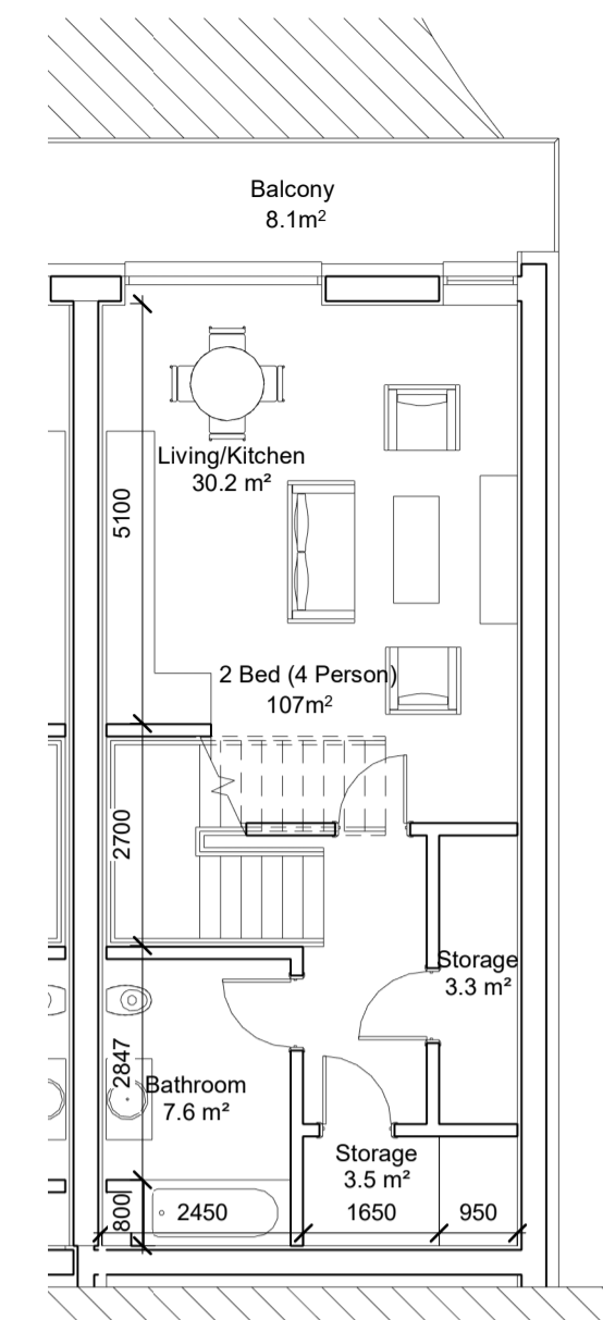
4 TH TYPE 3h (LG) 1 : 100 2B4P 107m² - Area 8.1m² - Private Amenity 115.8m² - TOTAL AREA
