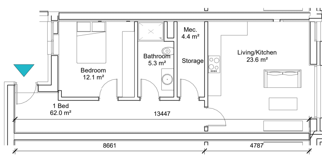
11 TH TYPE 7h (GF) 1 : 100 1B2P 61.4m² - Area 11.9m² - Private Amenity 73.3m² - TOTAL AREA
