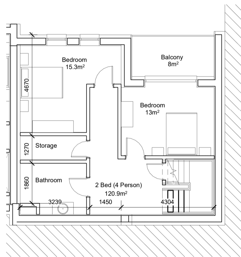
6 TH TYPE 4h (LG) 1 : 100 2B4P 120.9m² - Area 16m² - Private Amenity 138.9m² - TOTAL AREA
