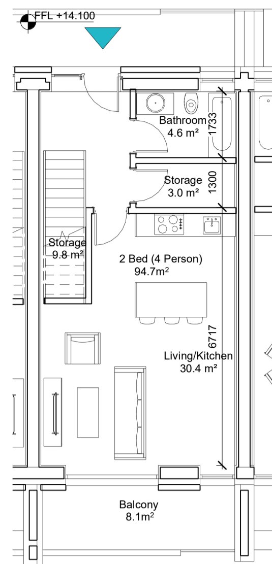
2 TH TYPE 2h (Lv01) 1 : 100 2B4P 94.7m² - Area 8.1m² - Private Amenity 102.8m² - TOTAL AREA
